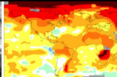
Climate Change
